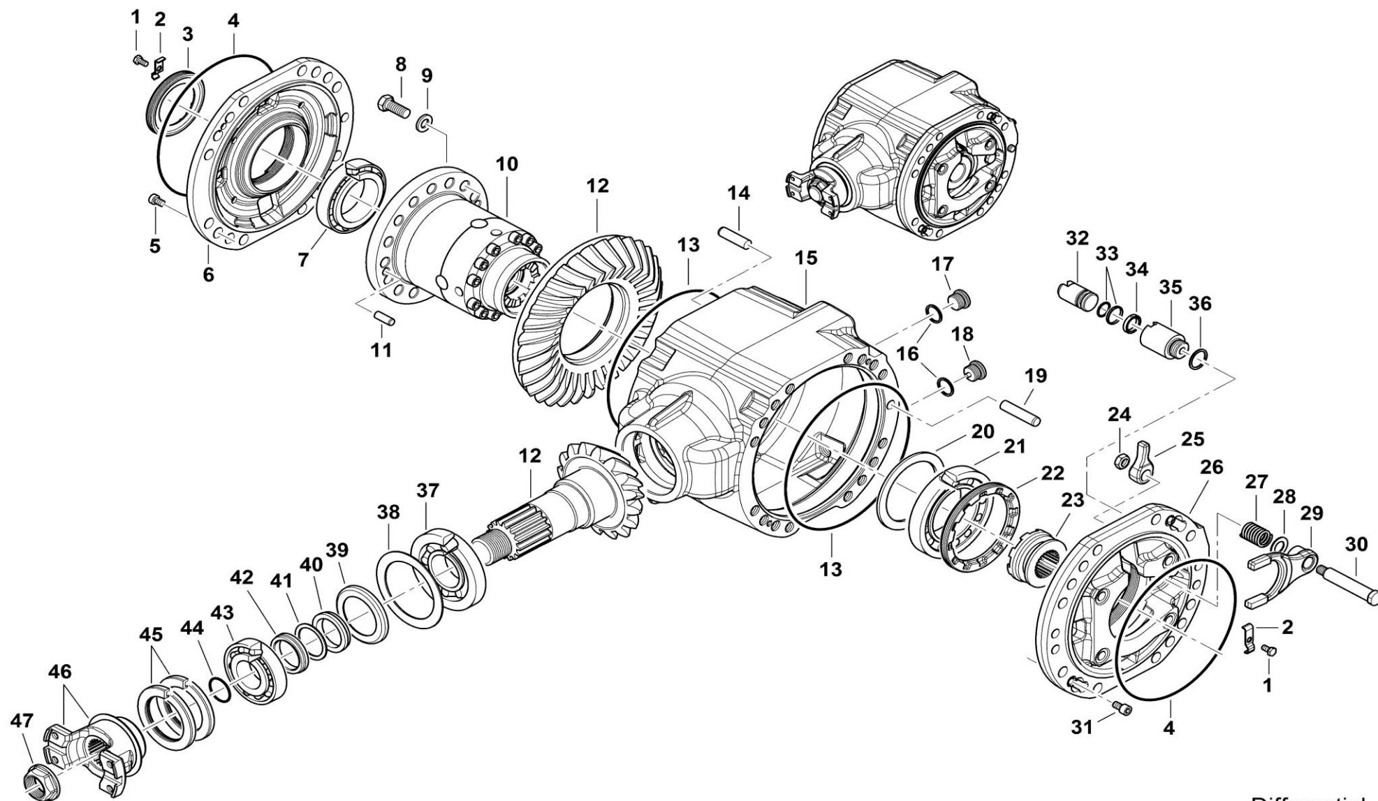
Differential 2401.228.A
