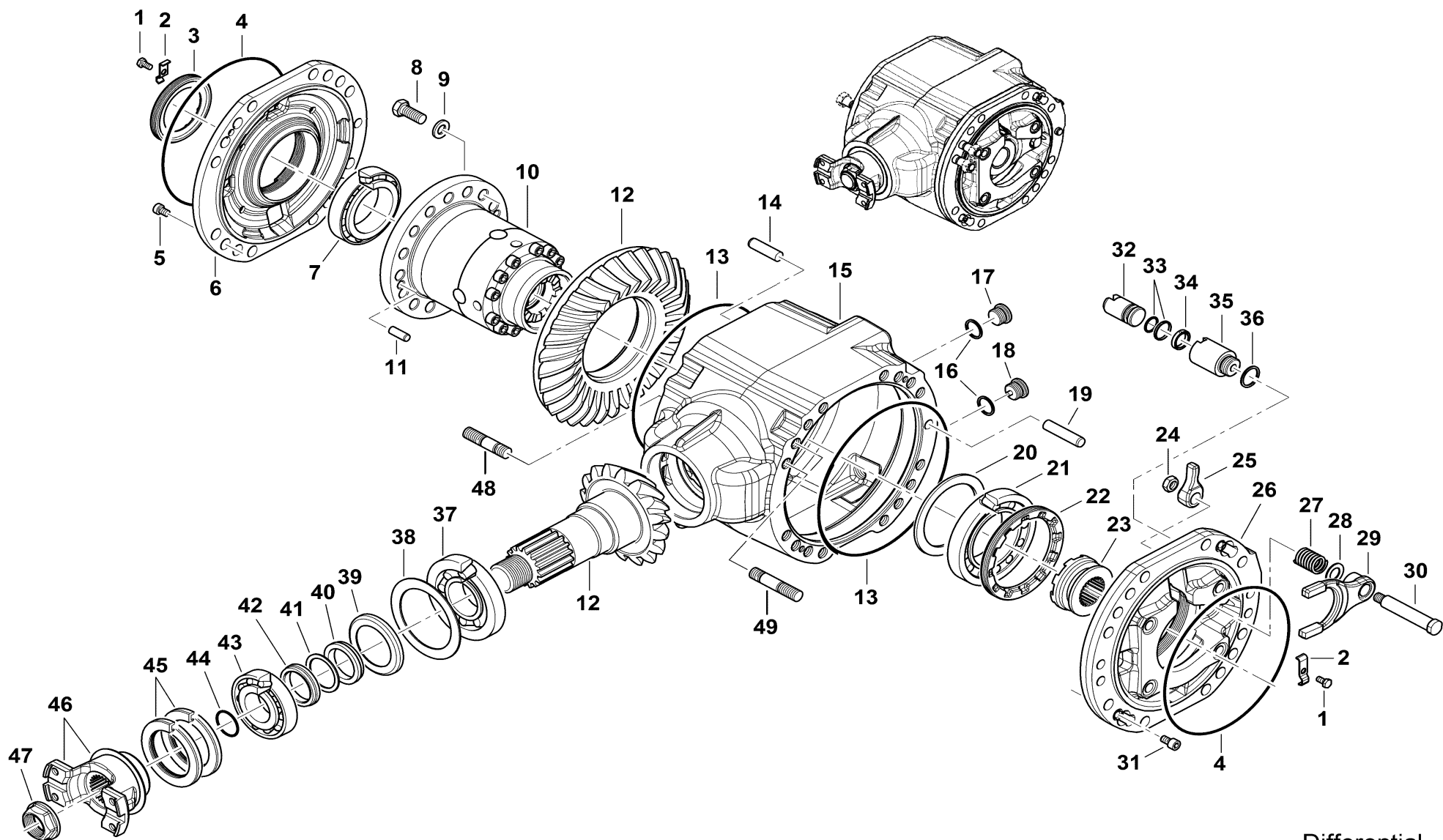
Differential 2401.228.B
